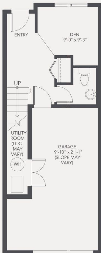
LOWER LEVEL
