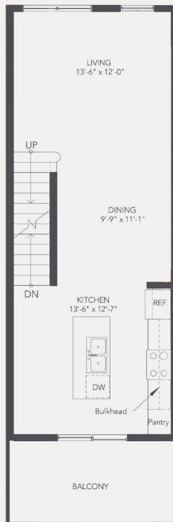
MAIN LEVEL
